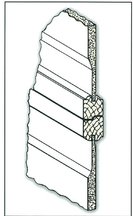
Below: cutaway of Cladwood Raised Panel Sections showing construction
